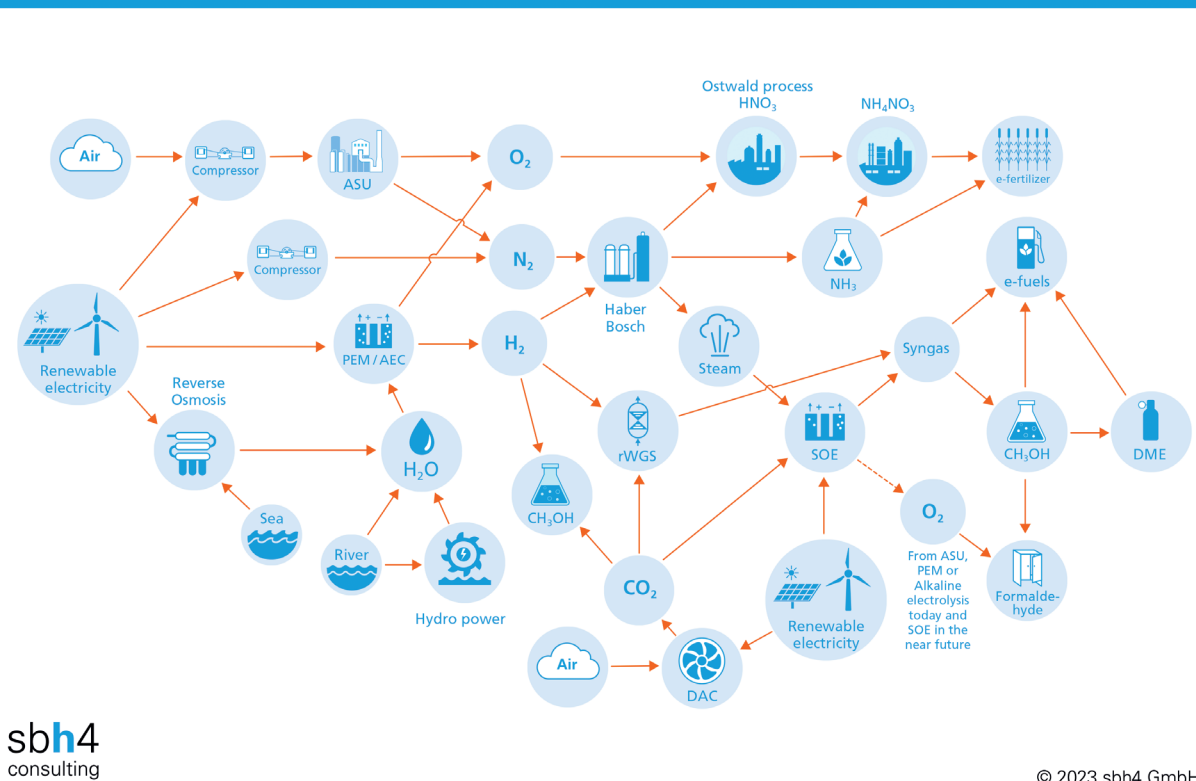
Air water and renewable power for e-fuels and e-fertilizers
