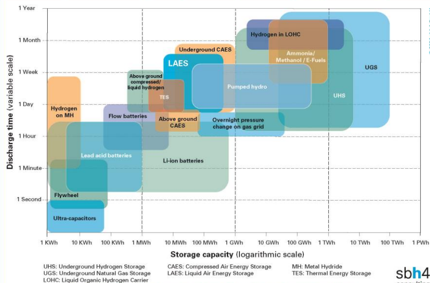
Renewable power and energy storage technologies, their capacity and discharge time
