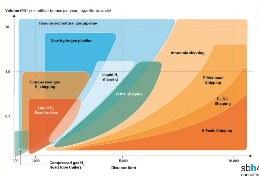
Hydrogen and hydrogen derivatives transport options when considering volume and distance
